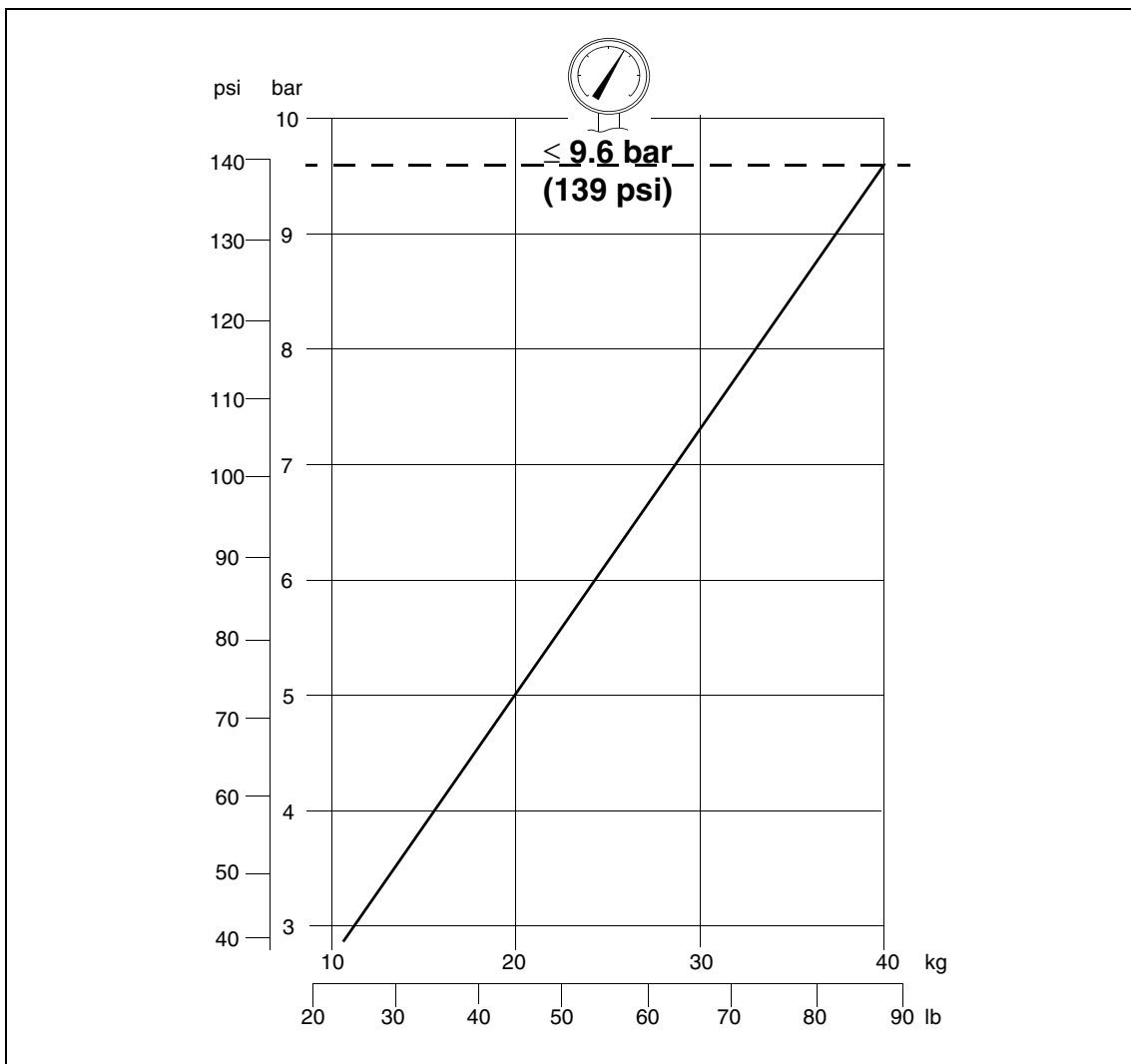
Fig 3 Pressurization Graph
